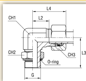
TIPO: EGC1061...4 ANELLO B4
