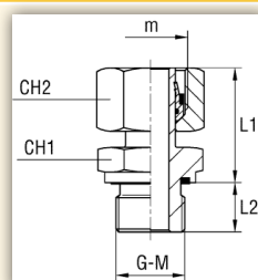
EGC1012...4 ANELLO B4
